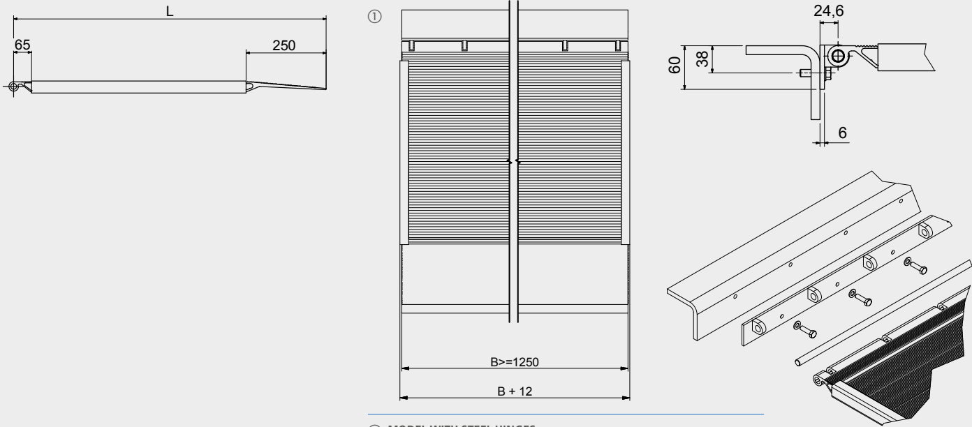
① MODEL WITH STEEL HINGES
