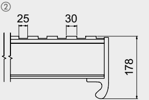
① STEP 50/50 (STANDARD) ② SPECIAL STEP 25/30 (ON REQUEST)
