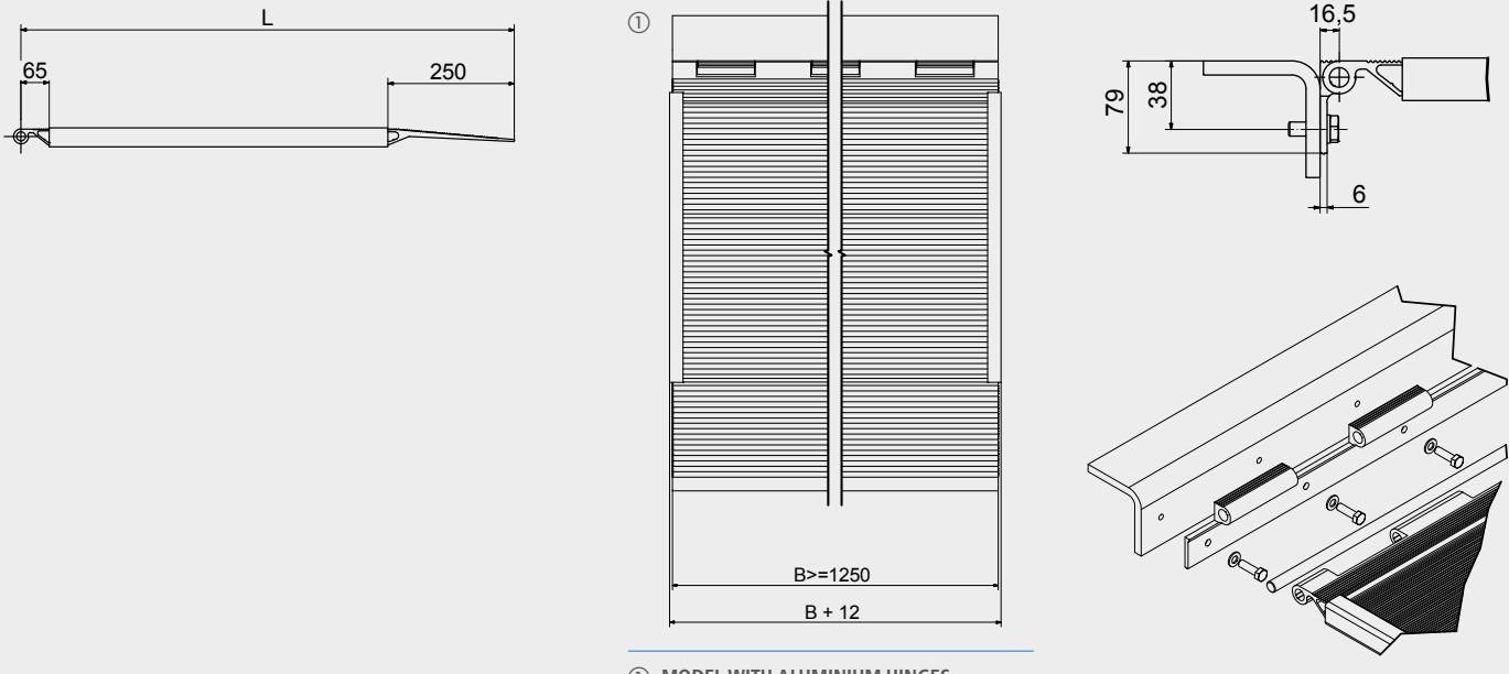
① MODEL WITH ALUMINIUM HINGES
