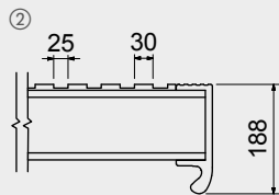
① STEP 50/50 (STANDARD) ② SPECIAL STEP 25/30 (ON REQUEST)
