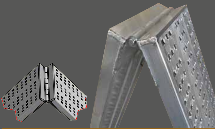
HINGED MODEL B3 (ON REQUEST)
