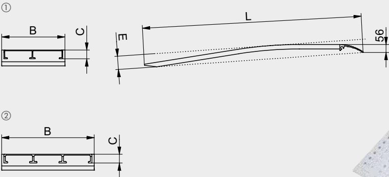
① MODEL B2 ② MODEL B3
